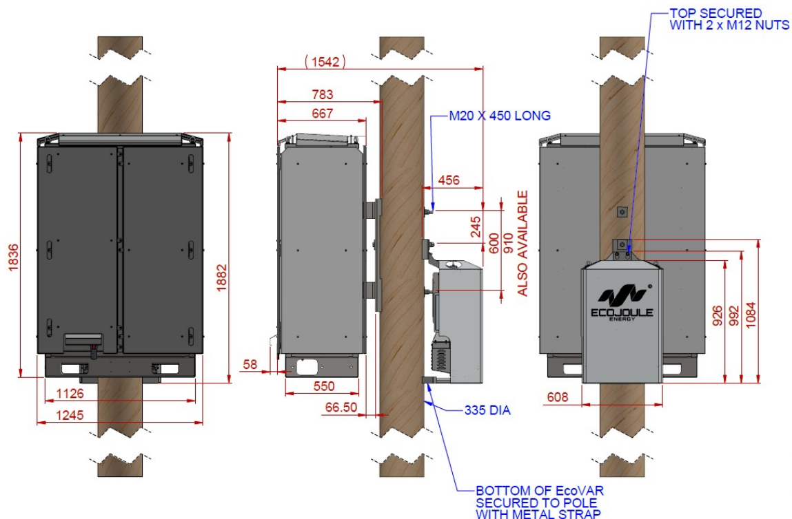
Mechanical dimensions (in mm)
